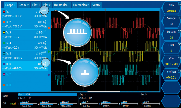
Scope display of the voltages at the converter output. The wideband values (u) show the PWM signal, the narrowband values (L) are sinusoidal.
